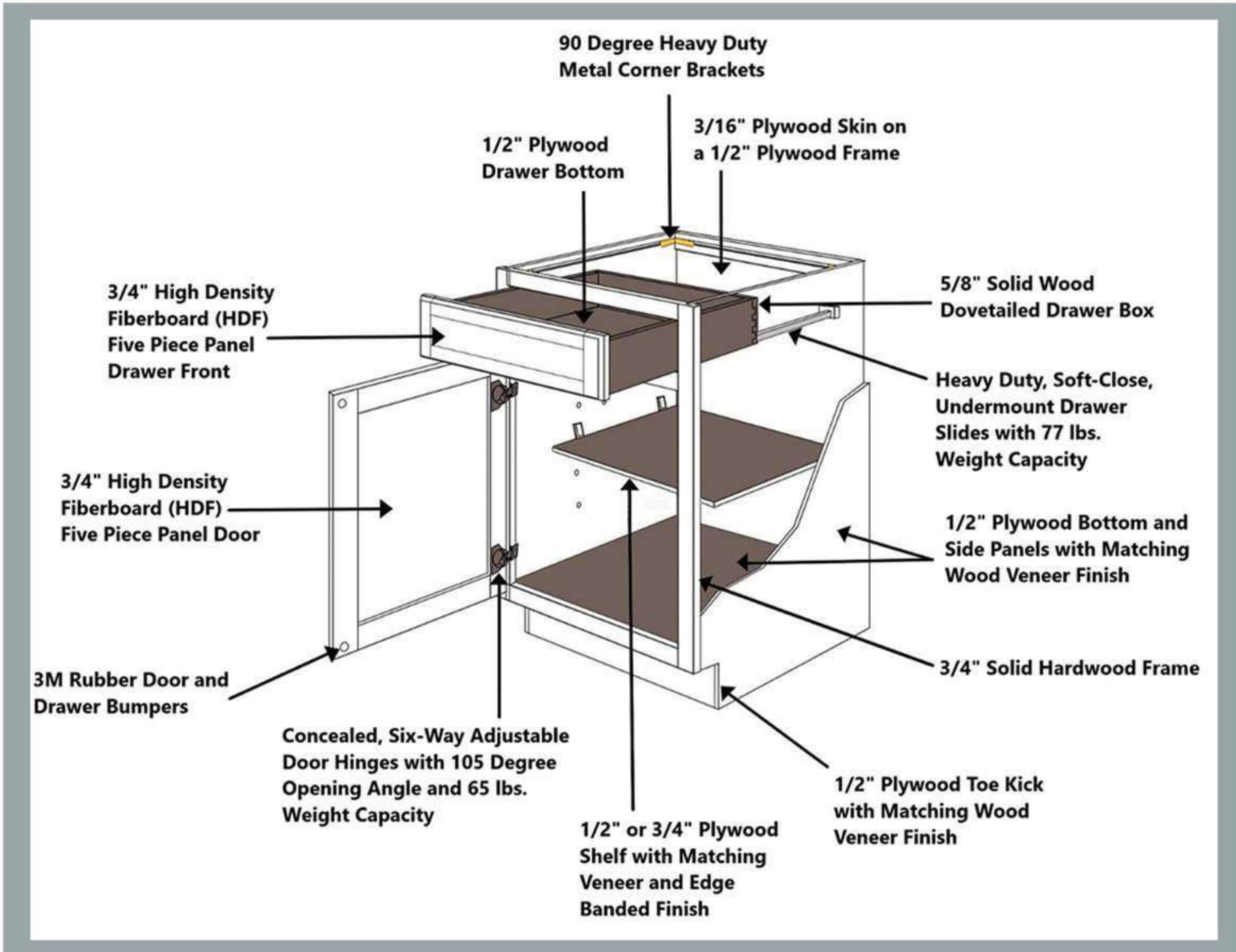
Base Cabinet Construction (HDF Door)
